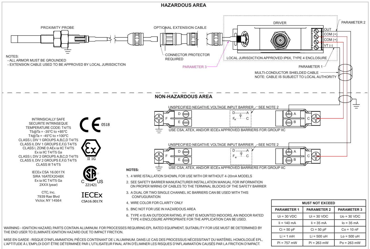
Figure 2. INS10060 - Four Wire Installation
