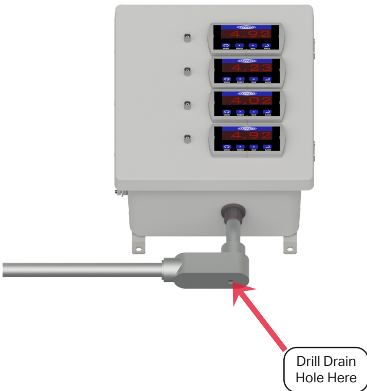
Figure 4. Conduit Entry for SCD111
