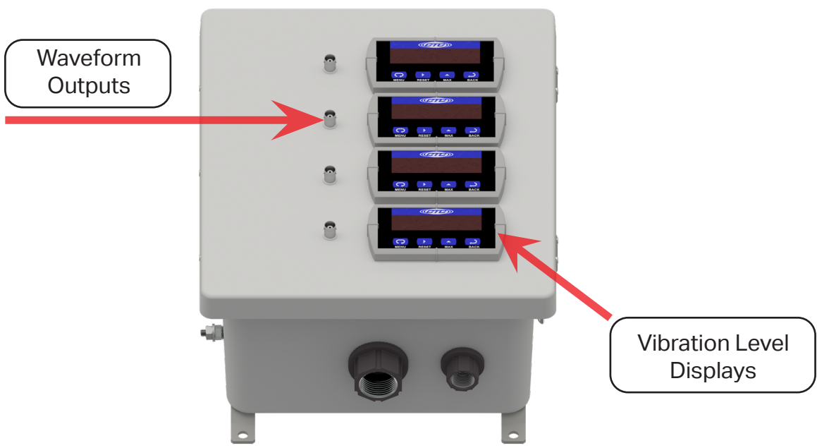
Figure 2. Diagram
