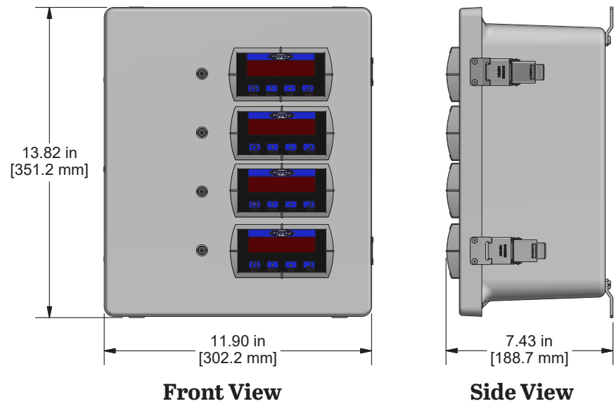
Figure 1. Dimensions
