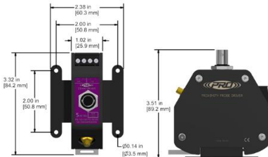
Figure 1 - 11mm Proximity Probe Driver
