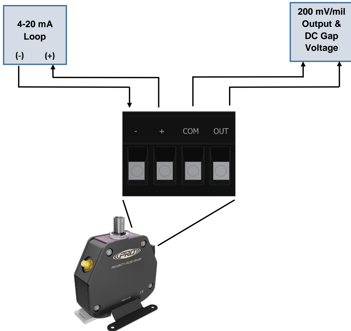
Figure 2 - Wire Connections
