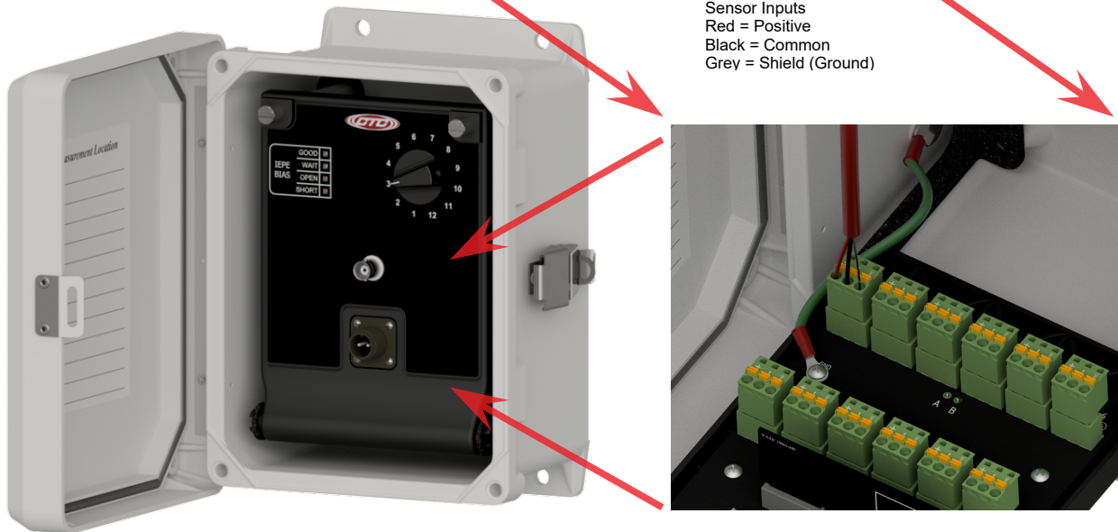
Figure 10. Field Wiring for 2-Conductor Sensor Inputs
