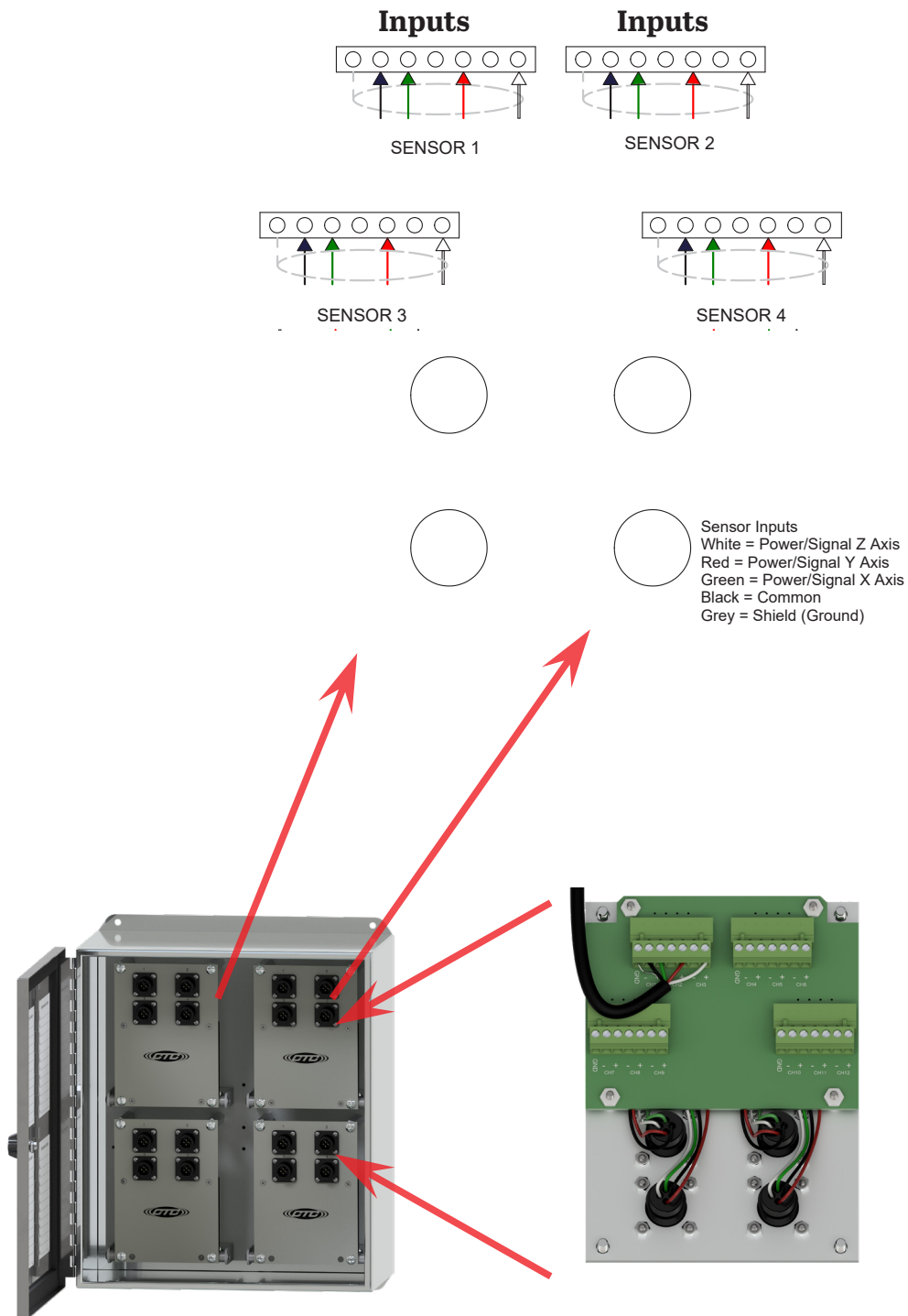
Figure 10. Field Wiring for 4-Conductor Triaxial Sensor Inputs
