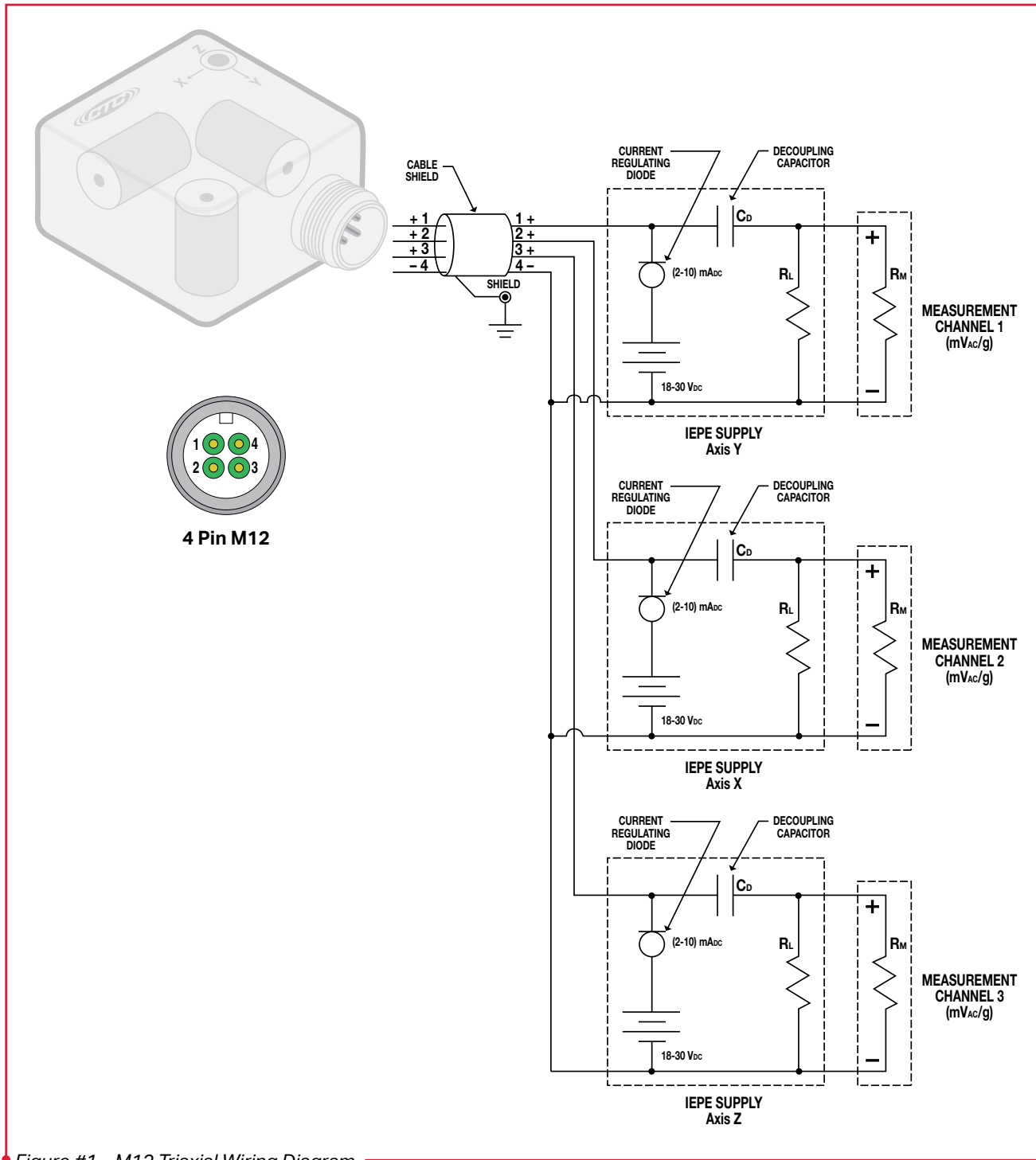
Figure #1 – M12 Triaxial Wiring Diagram
